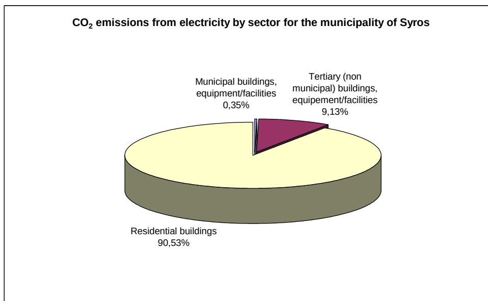
Figure 3.4. CO 2 emissions for electricity by sector in Syros for the year of 2001
