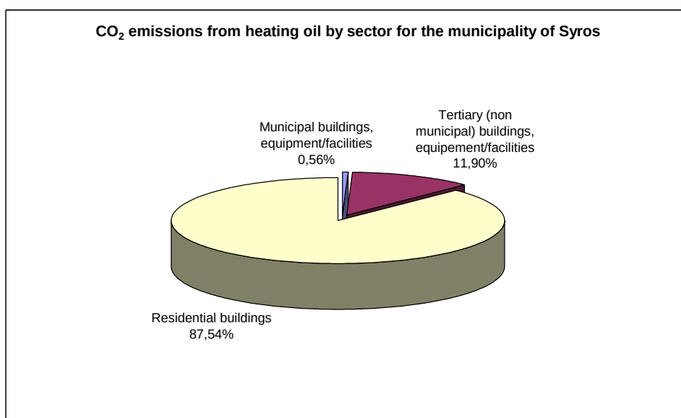
Figure 3.5. CO 2 emissions for heating oil by sector in Syros for the year of 2001
