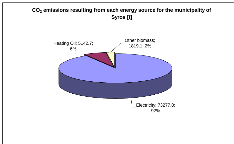
Figure 3.6. CO 2 emissions resulted from the energy sources in Syros for the year of 2001
